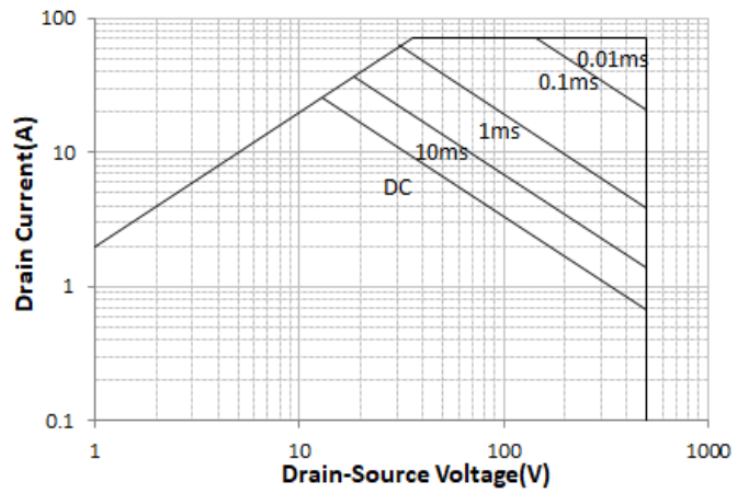
Maximum Safe Operating Area For MP18N50EI TO-220C
